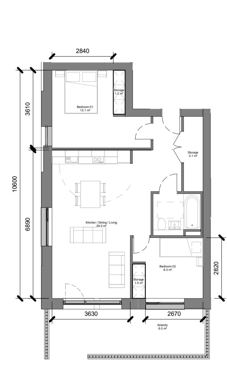
2B3P-Type B 1: 100
