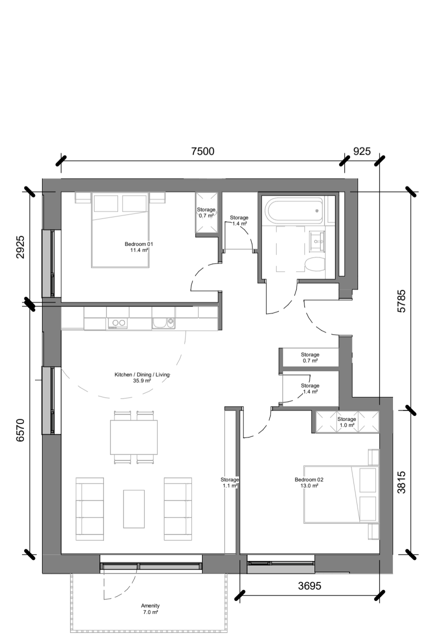
2B4P-Type G1 & G2 (Mirrored) 1: 100
