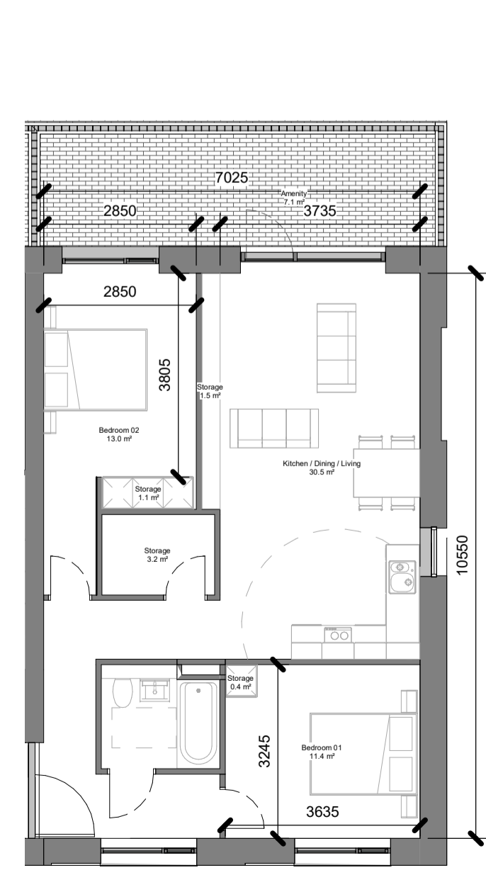
2B4P-Type D 1: 100
