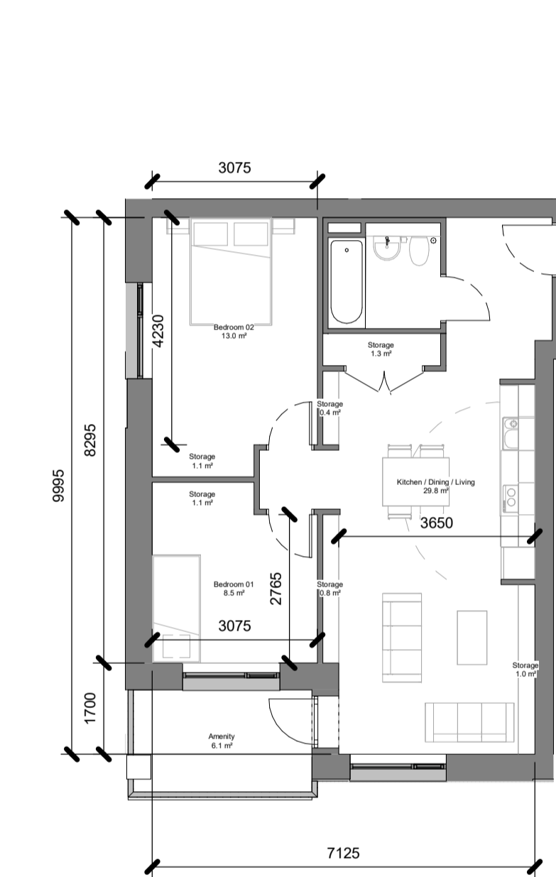
2B3P-Type C 1: 100
