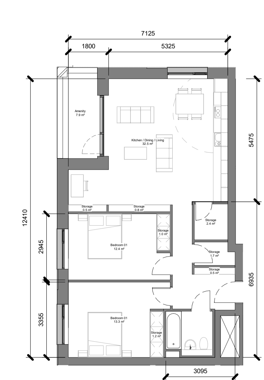
2B4P-Type F 1: 100
