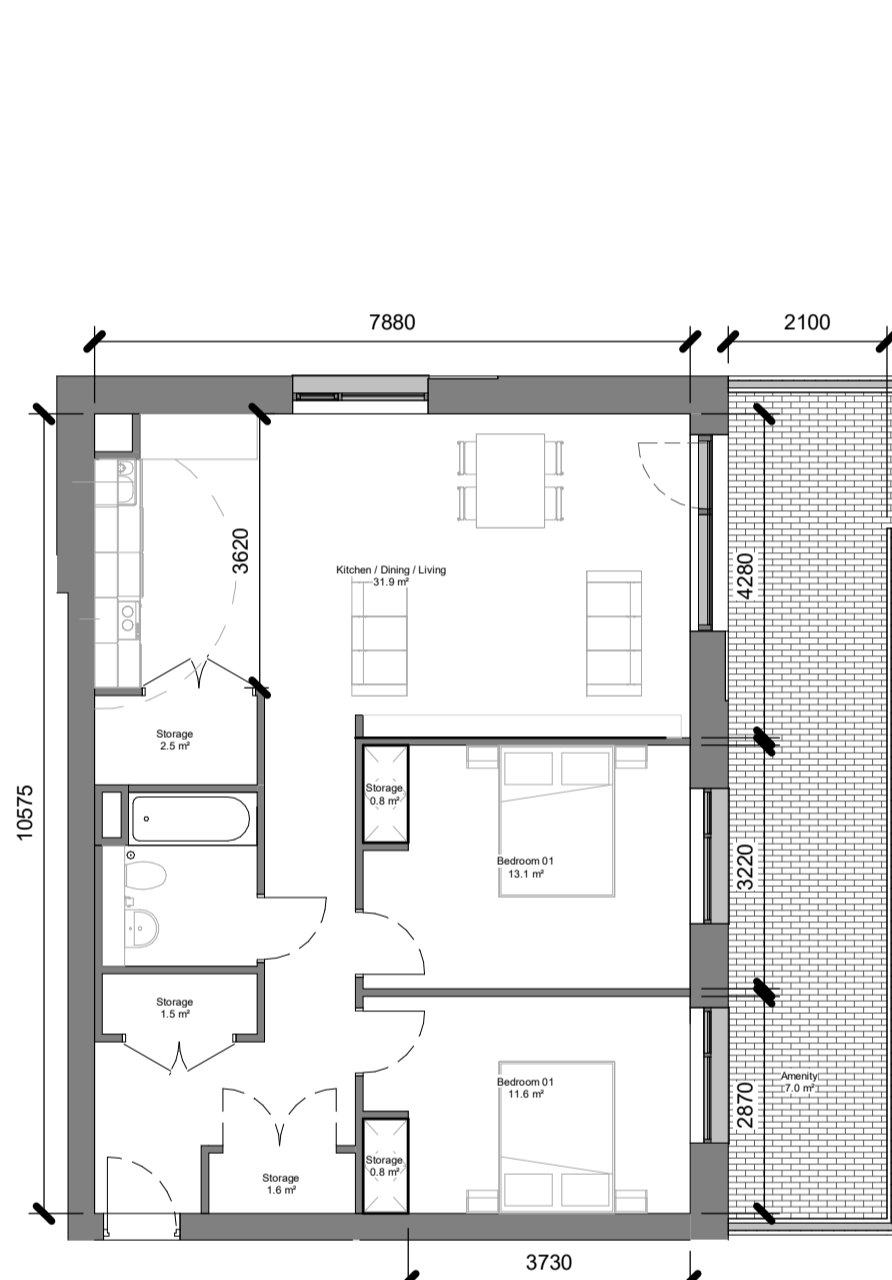
2B4P-Type B1 & B2 1B2P-Type (Mirrored) 1: 100
