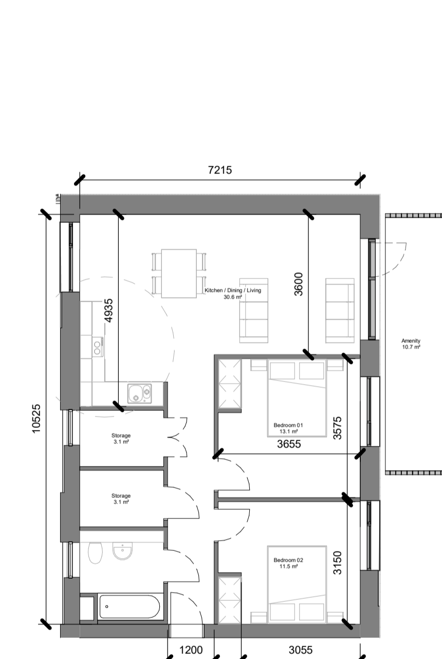
2B4P-Type A1 & A2 (Mirrored) 1: 100
