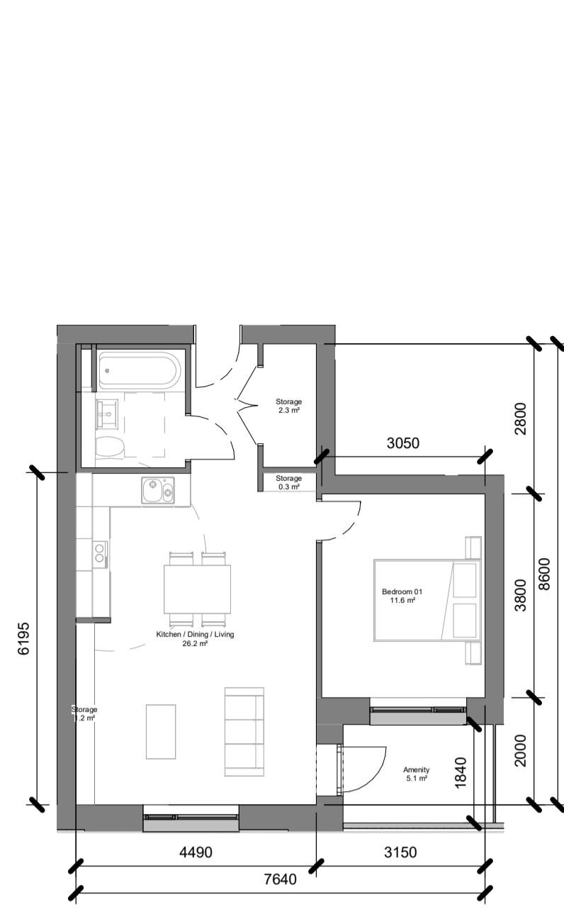
1B2P-Type M1 1: 100
