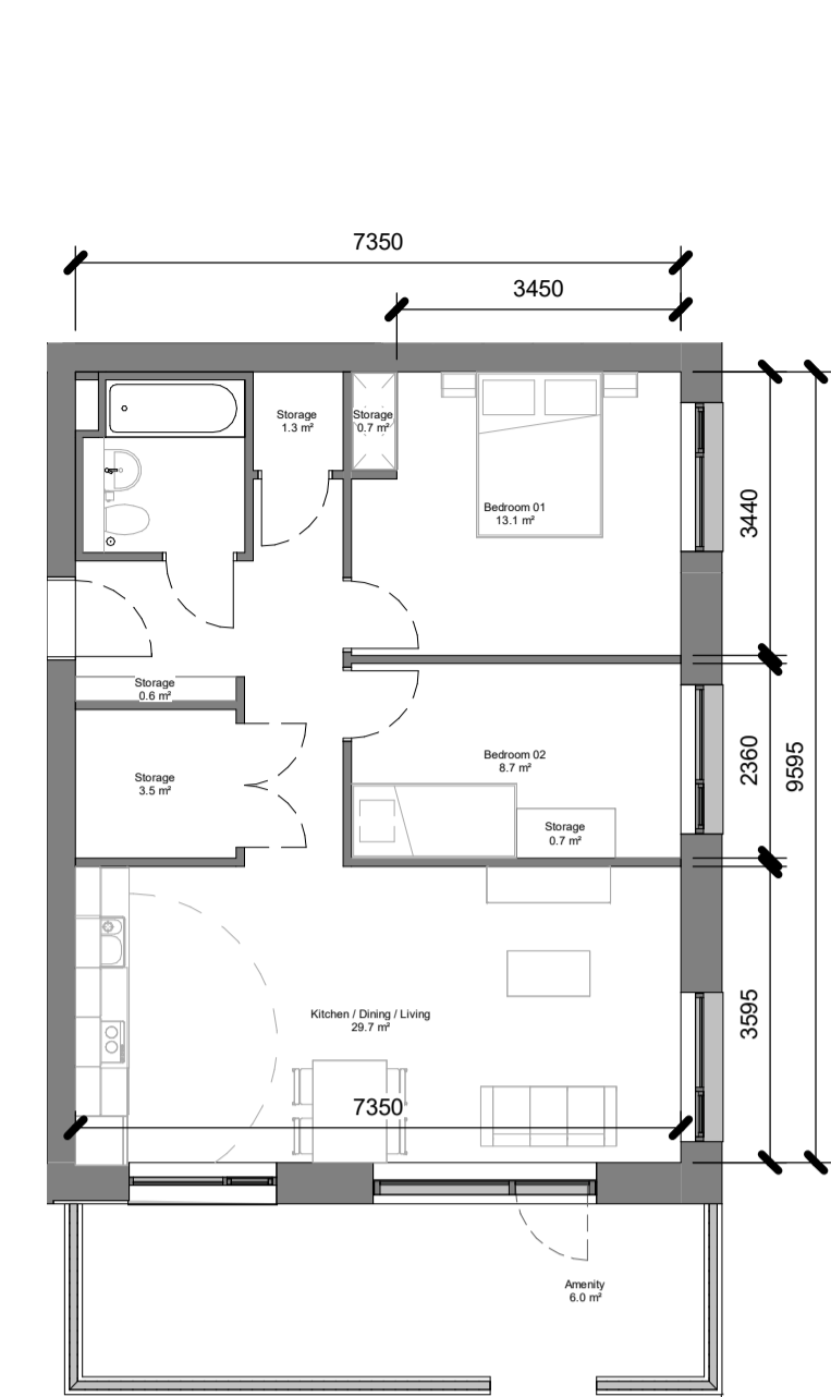
2B3P-Type A 1: 100
